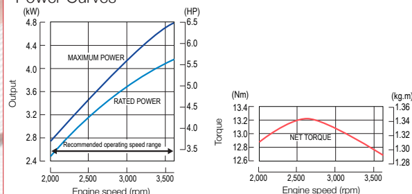
Power Curves
